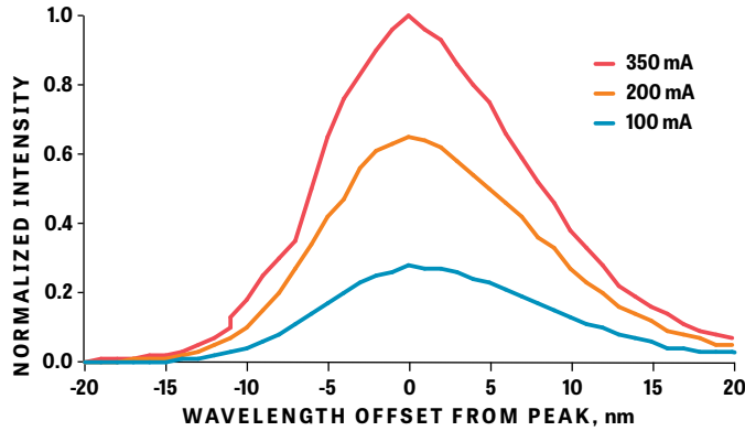
SPECTRUM OVER CURRENT
