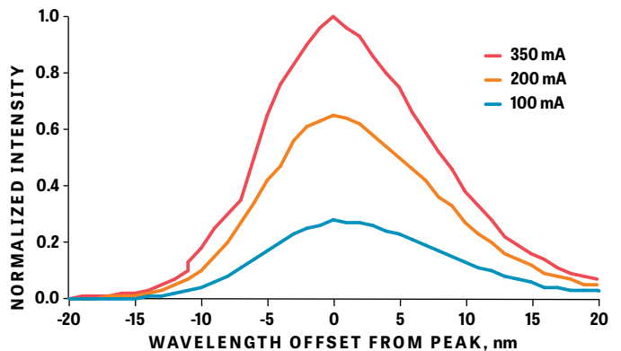
SPECTRUM OVER CURRENT
