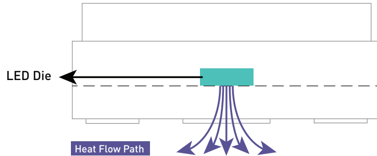
Schematic of Crystal IS Klaran LED Heat Flow Path.
