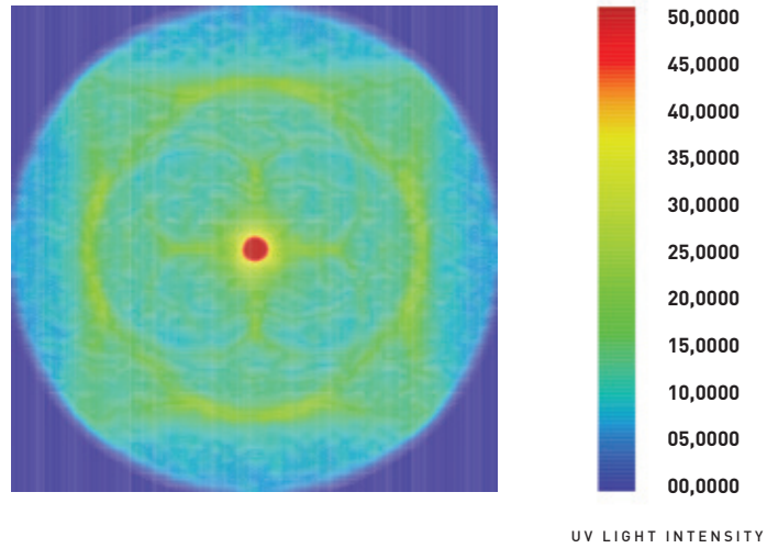
e-PTFE radiation pattern at 7.5 cm from end cap
