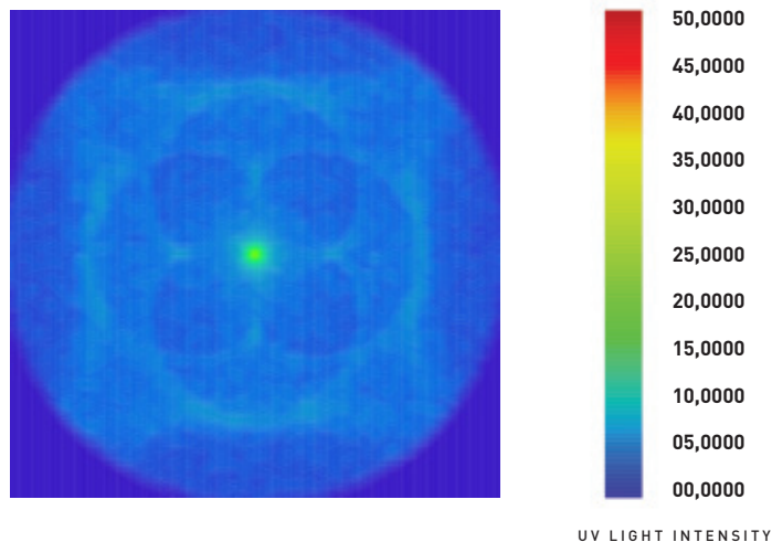
Stainless steel radiation pattern 7.5 cm from end cap
