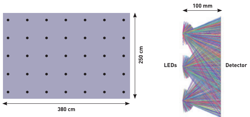
Arrangement of UVC LEDs in the duct
